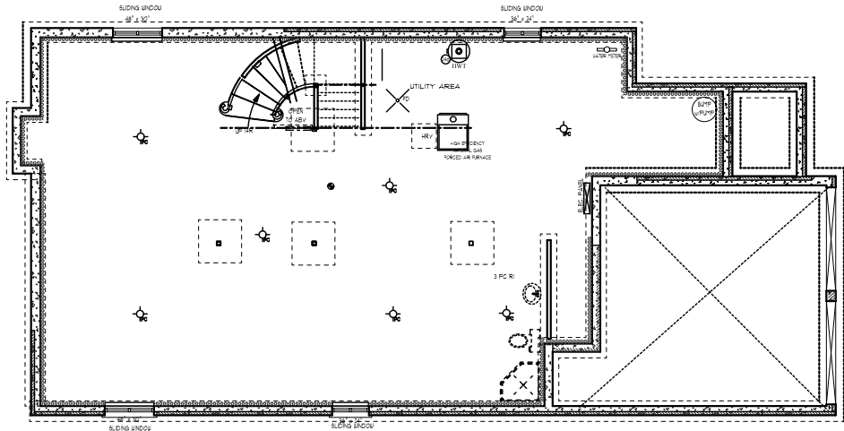
MICHELANGELO ELEV. A BASEMENT
